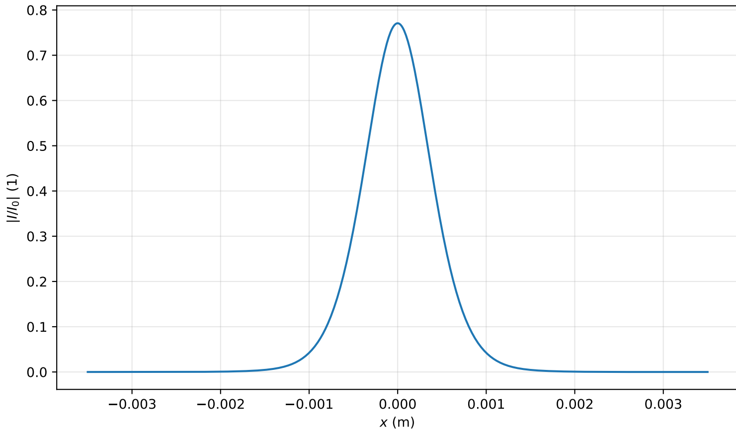
Intensity profile I(x, y = 0, z = 2.627m)/I_0 , P_{in}=0.6P_{cr} , artificial time
